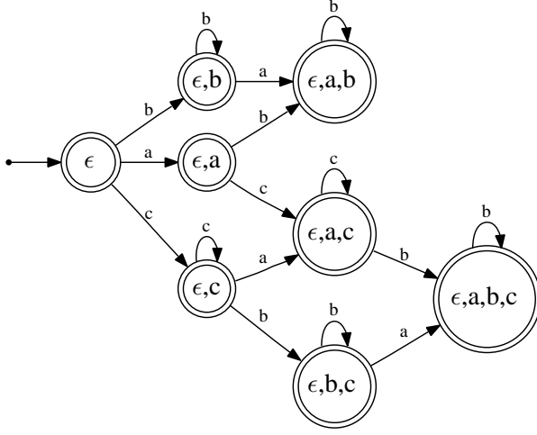
Figure 5: The DFA representation of the SP language given by \mathcal{G} = \langle \{a, b, c\}, \{aa, bc\} \rangle . Names of the states reflect subsets of subsequences up to length 1 of prefixes of the language. Note this DFA is trimmed, but not minimal.
