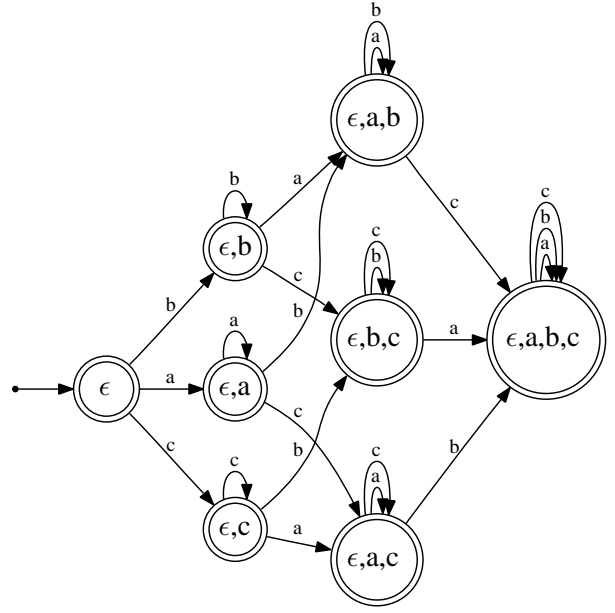
Figure 6: A DFA representation of the SP_2 language given by \mathcal{G} = \langle \{a, b, c\}, \Sigma^2 \rangle . Names of the states reflect subsets of subsequences up to length 1 of prefixes of the language. Note this DFA is trimmed, but not minimal.
