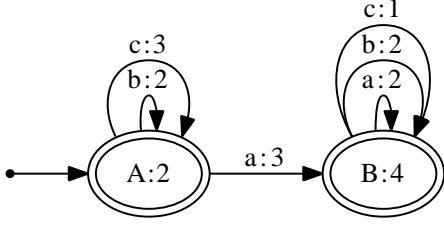
Figure 2: The automata shows the counts obtained by parsing \mathcal{M} with sample S = \{ab, bba, \epsilon, cab, acb, cc\} .
